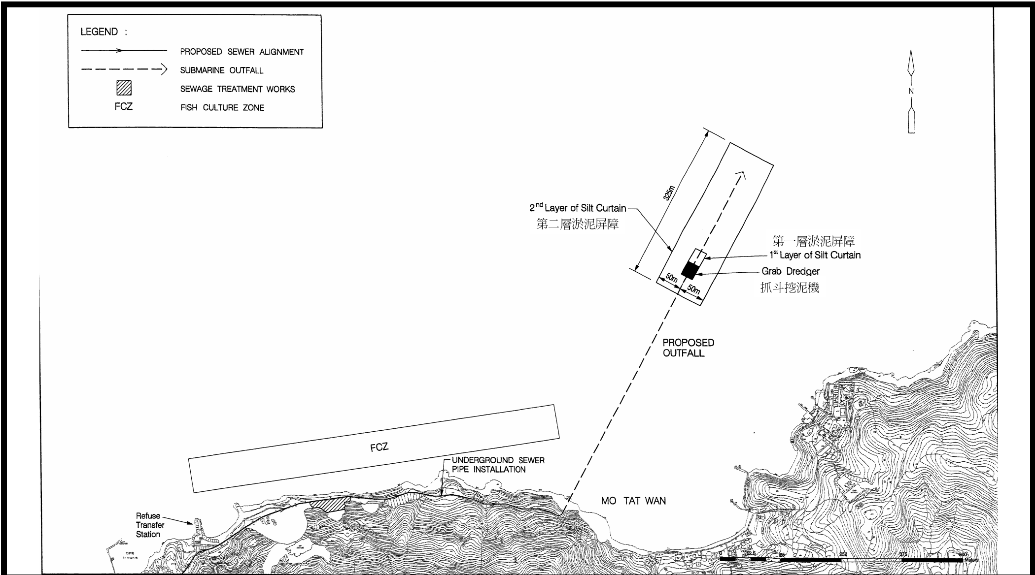
Figure 3: Arrangement of Silt Curtain during Construction
